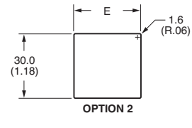
Panel Cutouts
