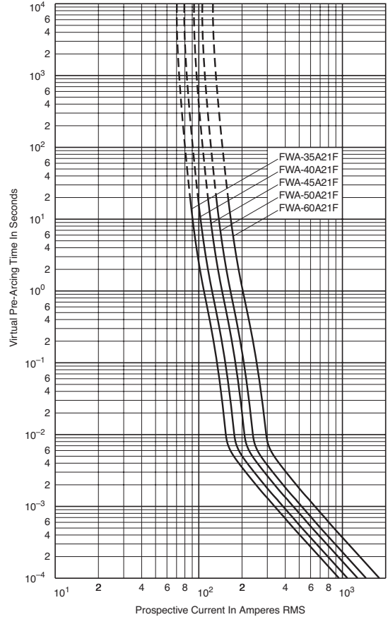
Time-Current Curve
