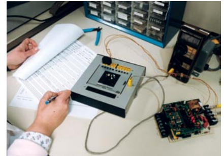
Individual components are tested to ensure that temperature specifications are not exceeded.
